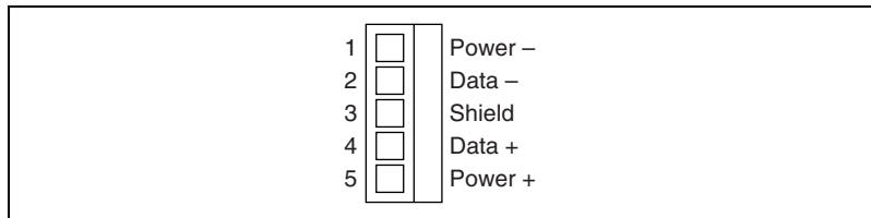
Figure B-3. Screw Terminal Block Pinout
