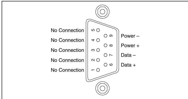
Figure B-2. Fieldbus Connector Pinout
