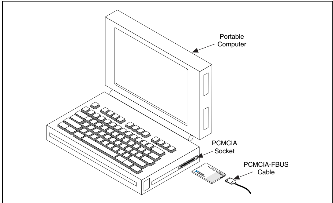
Figure 2-1. Inserting the PCMCIA-FBUS
